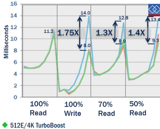
Figure 4 – Iometer results for 4K block size 100% random I/O
