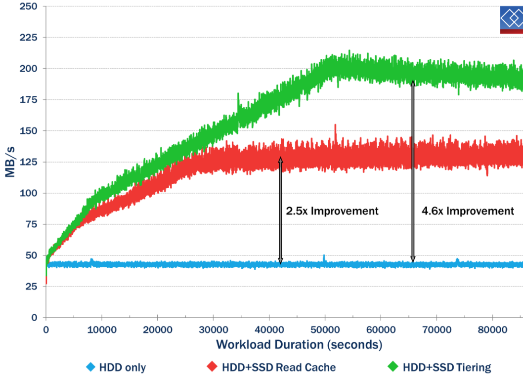
MB per Second of Total Storage Bandwidth
