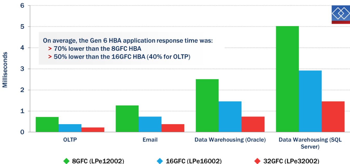
Average I/O Response Time by Blocksize (lower is better)
